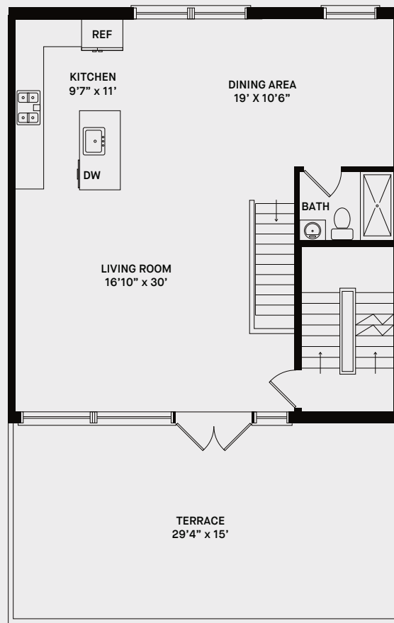
FOURTH FLOOR
